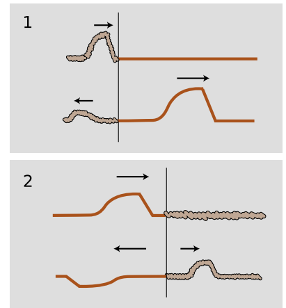
e / 1. An uninverted reflection. The reflected pulse is reversed front to back, but is not upside-down. 2. An inverted reflection. The reflected pulse is reversed both front to back and top to bottom.
