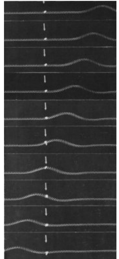
e / As the wave pulse goes by, the ribbon tied to the spring is not carried along. The motion of the wave pattern is to the right, but the medium (spring) is moving up and down, not to the right.
