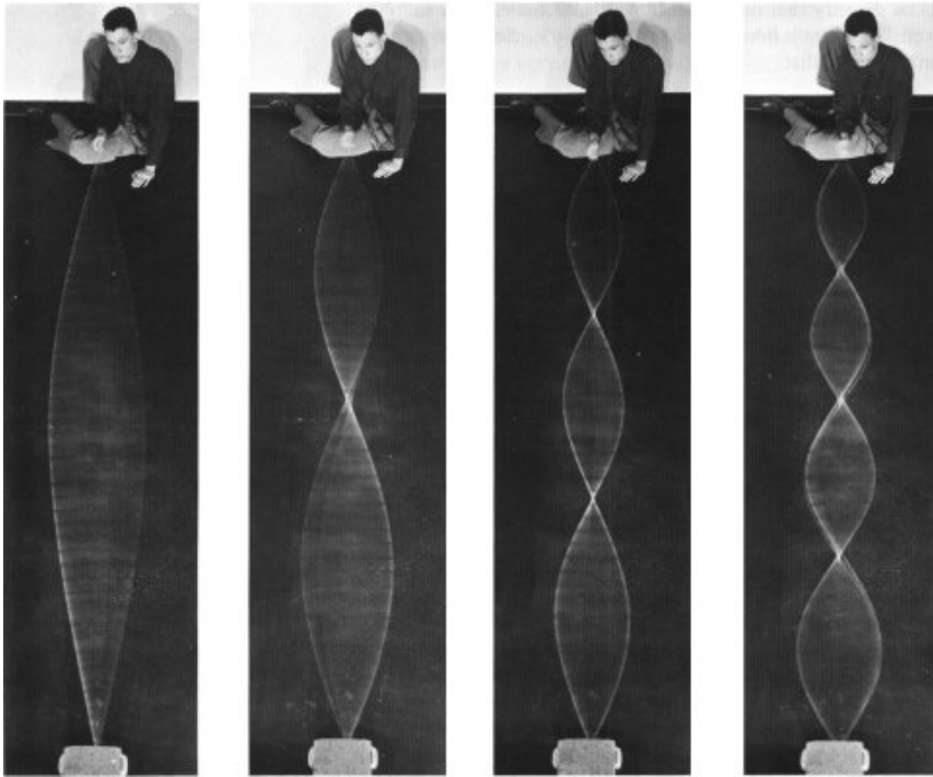
t / Standing waves on a spring.
